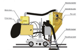
Flux Recovery System
